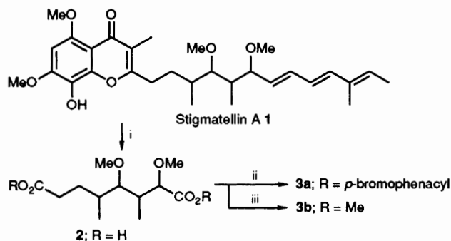
Scheme 1 Stigmatellin A and degradation studies. 1 Reagents and conditions: i, O 3 , NaOH, H 2 O 2 ; ii, 2,4'-dibromoacetophenone; iii, diazomethane.
